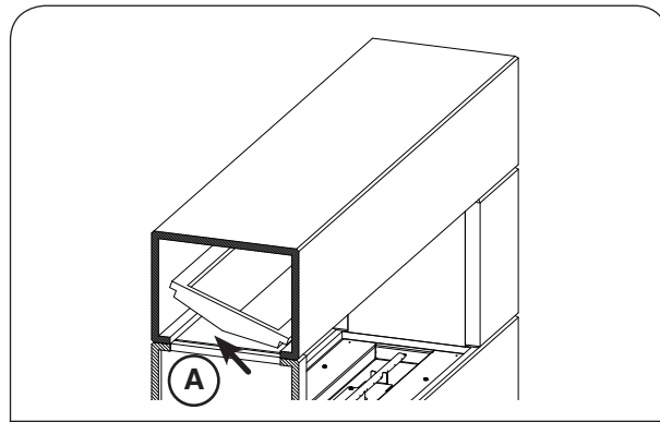
Fig. 21-1 Install side liners
