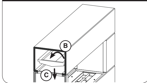
Fig. 21-2 Install top liner
