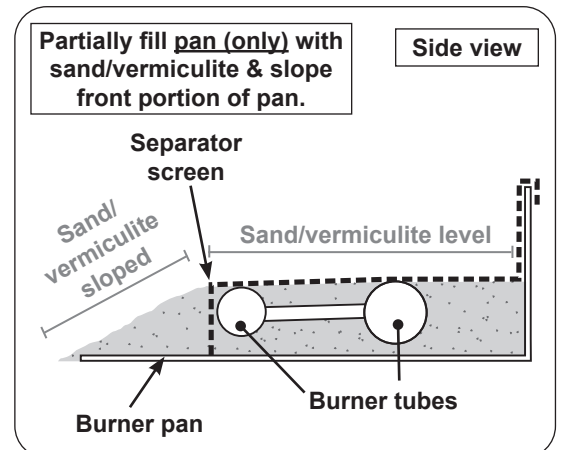
Fig. 12-3 Sand/vermiculite & screen detail
