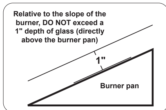
Fig. 13-2 Proper media placement
